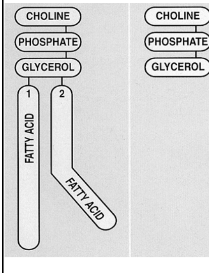
Figure 2. Oil-phase versus water-phase phospholipids. Lt: PC (phosphatidylcholine). Rt: GPC, lacking the fatty acid “tails” of PC.
